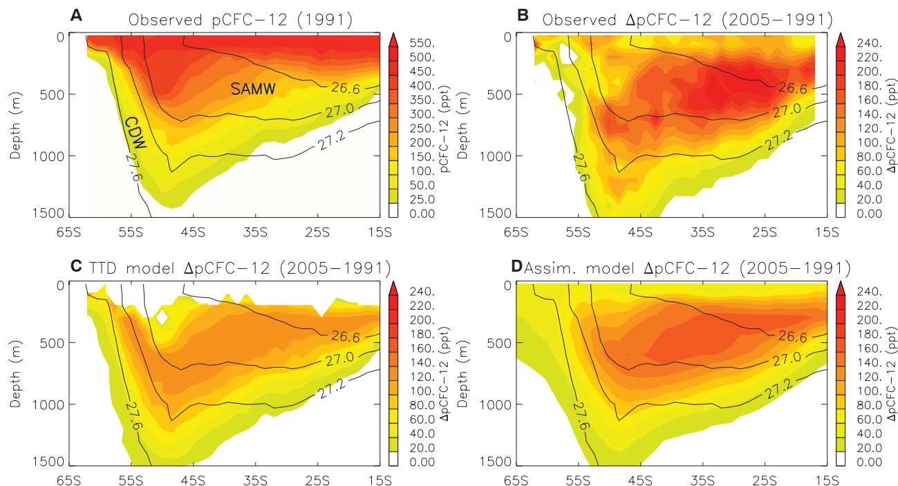
Fig. 1. Depth-latitude cross sections for WOCE P16 section (~150°W; see Fig. 2A): (A) observed p CFC-12 in 1991. Changes in p CFC-12 between 1991 and 2005 for (B) observations, (C) TTD model, and (D) assimilated model. Contours show potential density referenced to the sea surface \sigma_0 ( \text{kg/m}^3 ). ppt, parts per thousand.
