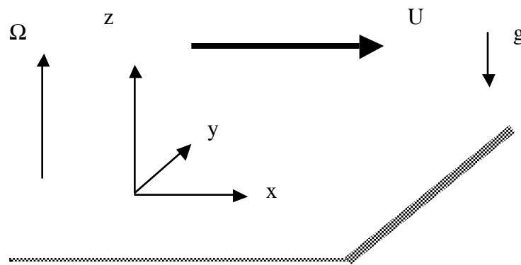
Figure 5.1.1 The fluid flows in the x direction with speed U far from a solid wall at z=0 .
