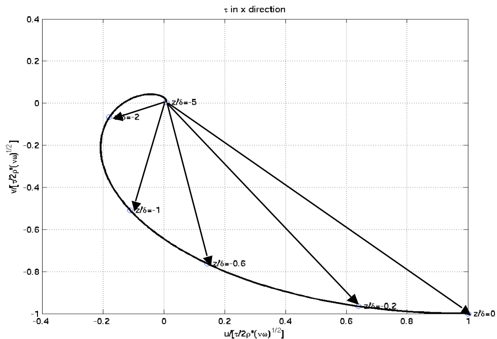
Figure 5.2.3 a The Ekman spiral below a stress in the x direction.
