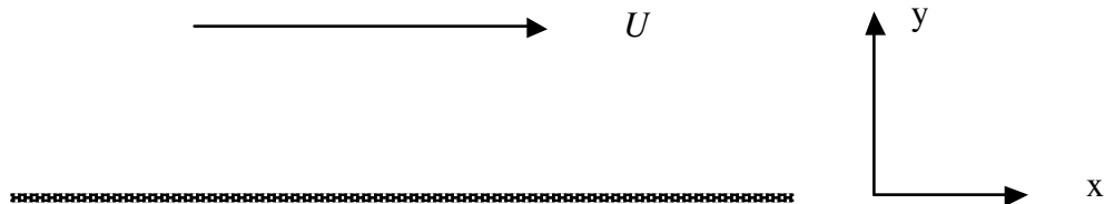
Figure 5.3.1 A uniform flow in the x direction at t=0 must satisfy the no slip condition at y=0 .
