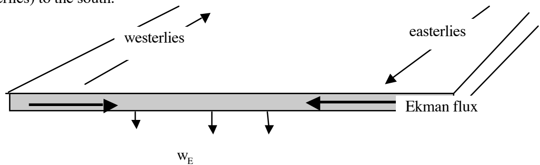
Figure 5.2.5 The wind system in the region of the subtropical gyre produces a convergence of the Ekman flux and a downward vertical velocity w_E that is responsible for driving the major oceanic gyres.
