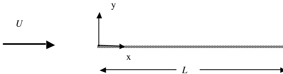
Figure 5.4.1 A uniform flow approaches a solid plate of length L .
