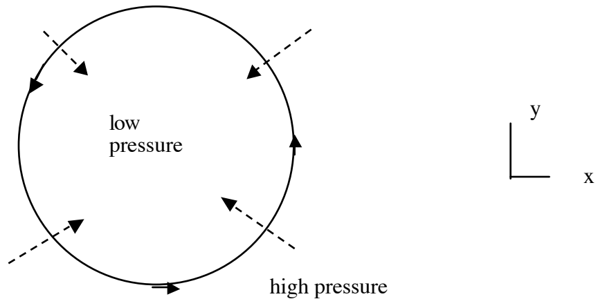
Figure 5.1.6 A circular cyclonic flow ( counter clockwise) showing the direction (dashed arrows) of the cross isobar flow. In the figure the isobars are coincident with the direction of the circular flow far from the solid surface.
