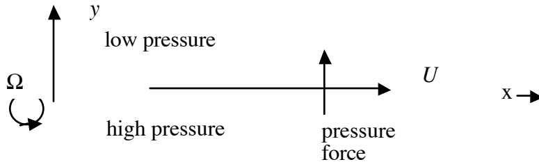
Figure 5.1.2 The balance between the pressure gradient and the Coriolis acceleration in the solution ((5.1.5)).
