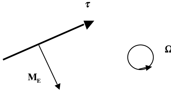
Figure 5.1.5. The relation between the applied stress on the fluid and the resulting Ekman mass flux (plan view).
