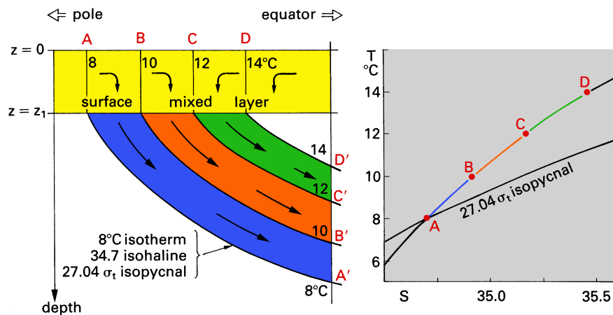
Fig. 5.3. Sketch of water mass formation by subduction in the Subtropical Convergence. The T-S diagram shows both the meridional variation of temperature and salinity between stations A and D , and the vertical variation equatorward of station D from the surface down along the line A'B'C'D' . For more detail, see text.
