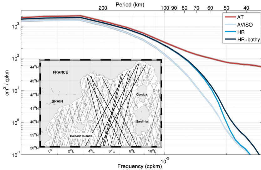
Figure 1. The mean power spectra of the SLA in the NWMed for the different products, with the 95% confidence interval shaded in gray (error was estimated using chi-square test). In dark red is the along-track 1 Hz data while the gridded fields are in blue, the lighter being the AVISO product and the darker ones are the HR products. The spectrum for these datasets was computed from SLAs interpolated at the track locations. The fitted slopes between 70 and 250 km are indicated for each spectrum. Bottom left corner: map with the position of the tracks (the long tracks used for the spectra computation are shown in black, and the others are shown in gray).
